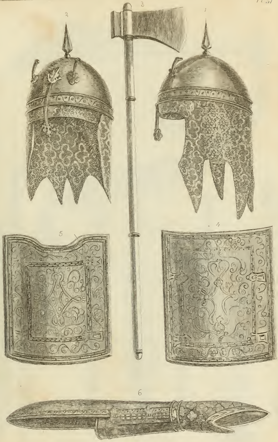
Asiatic Armour.
